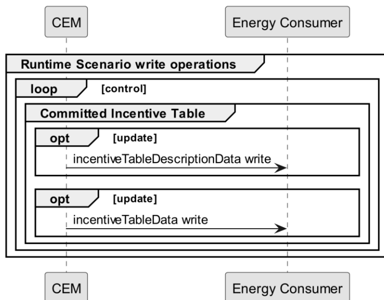
1722 Figure 25: Scenario 2 - Runtime Scenario write operations
