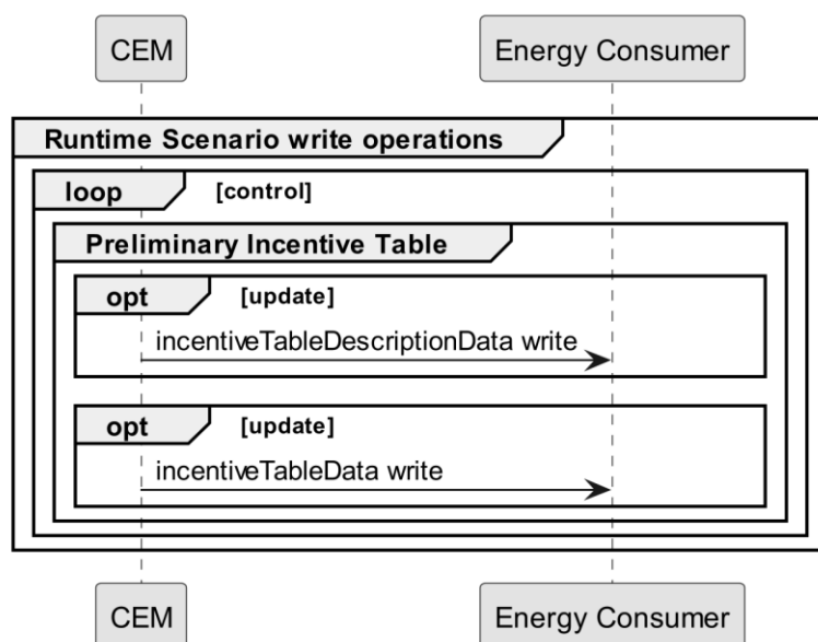
2007 Figure 28: Scenario 3 - Runtime Scenario write operations
