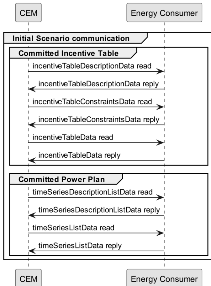
Figure 23: Scenario 2 - Initial Scenario communication sequence diagram
