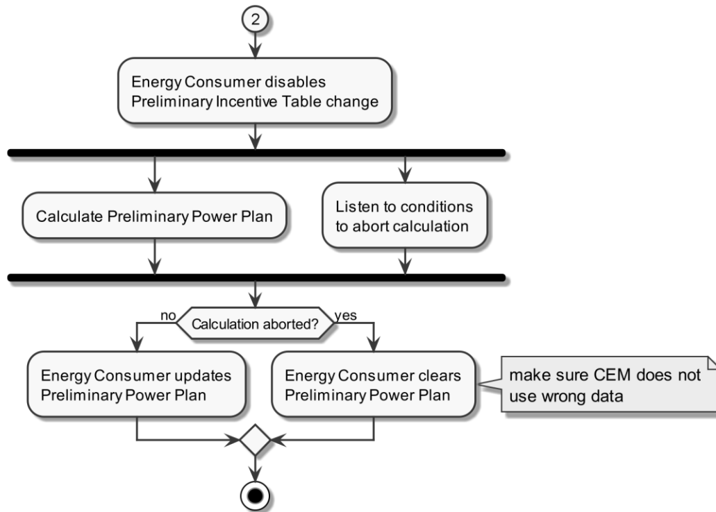
Figure 13: Activity branch "Update of Preliminary Power Plan" diagram of Scenario 3
