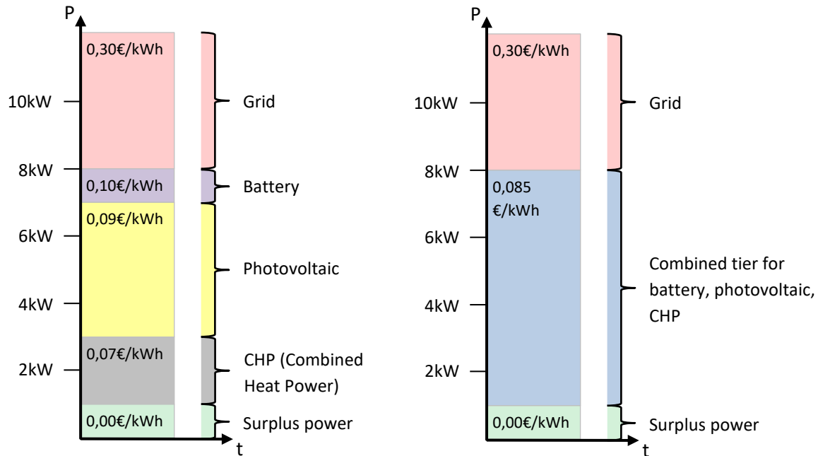
Figure 5: Example for five tiers and "compression" to three tiers
