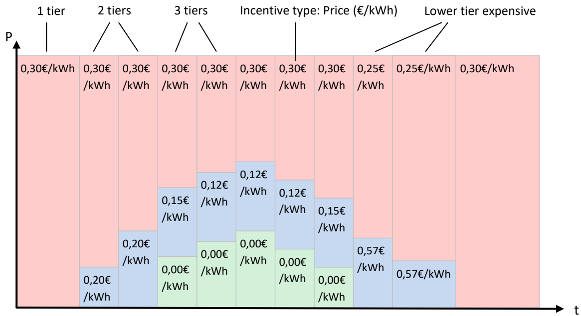
Figure 2: Incentive Table example: Power (P) dependent incentives over time (t)
