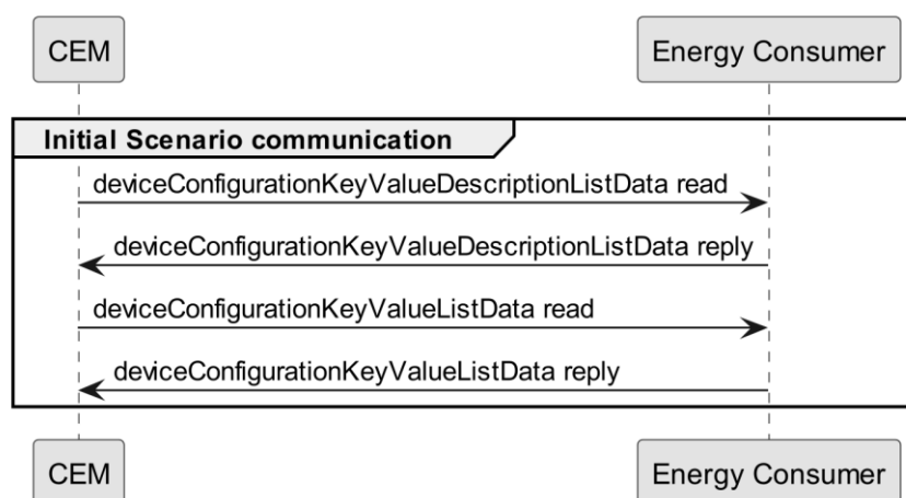
1572 Figure 21: Scenario 1 - Initial Scenario communication sequence diagram
