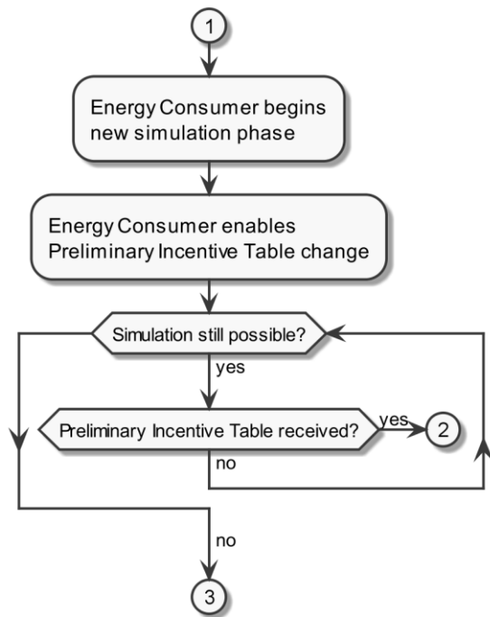
Figure 12: Activity begin diagram of Scenario 3
