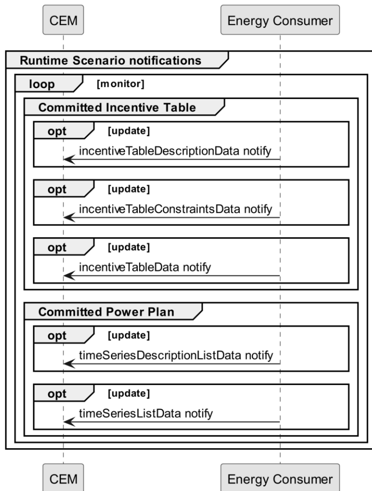
Figure 24: Scenario 2 - Runtime Scenario notifications
