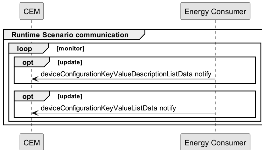
Figure 22: Scenario 1 - Runtime Scenario notifications
