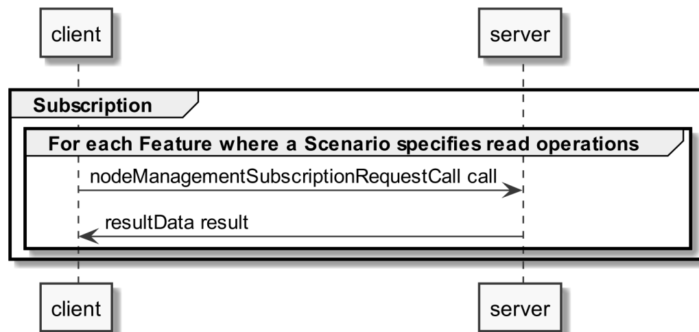
Figure 20: Pre-Scenario communication - Subscription sequence diagram
