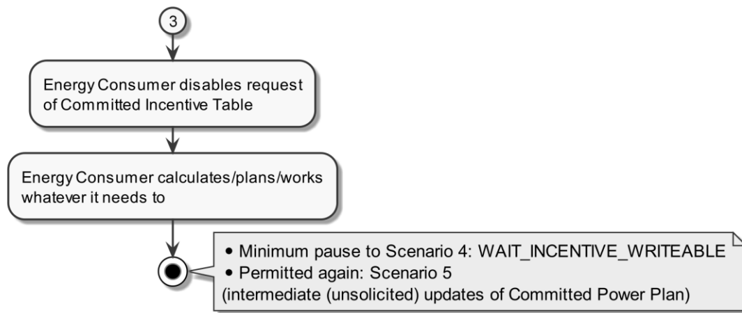
Figure 10: Activity branch "Autonomous operation" diagram of Scenario 2
