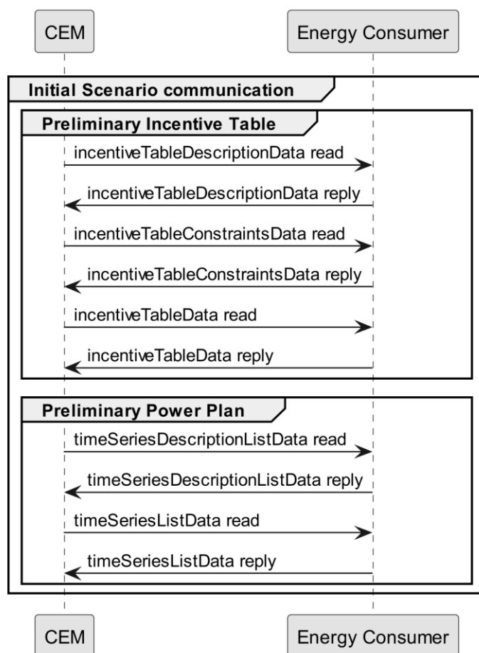
1948 Figure 26: Scenario 3 - Initial Scenario communication sequence diagram
