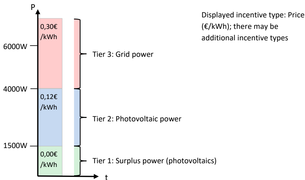
Figure 3: Single slot of an Incentive Table with three example tiers
