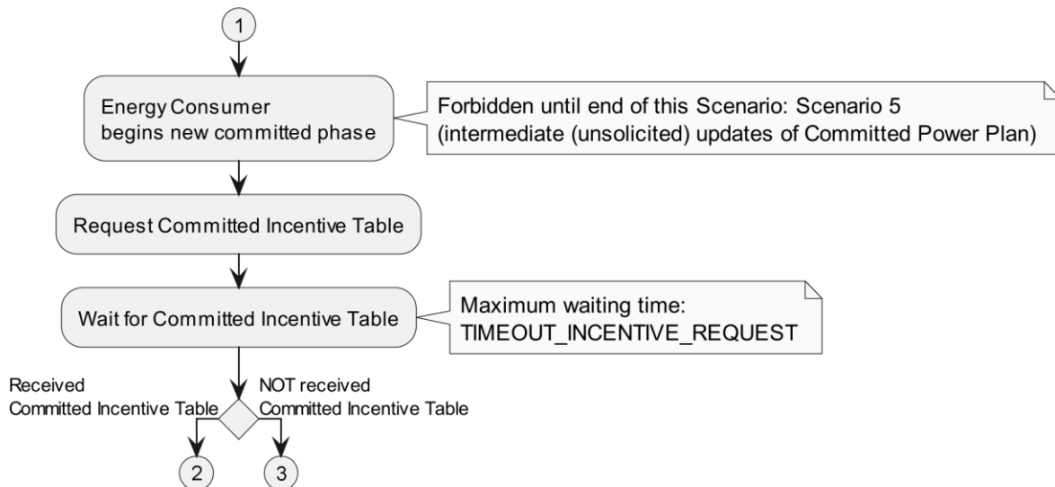
Figure 8: Activity begin diagram of Scenario 2
